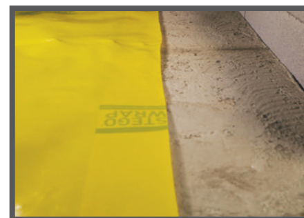
Note: The distance to which the vapour barrier is extended adjacent to, onto, or completely over a footing or grade beam should be determined by the project design team.
