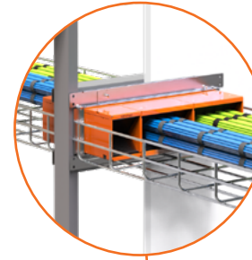
High-density solutions Series 84+ in combination with Series 44+
