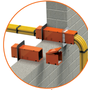
Extensions For use with thicker walls
