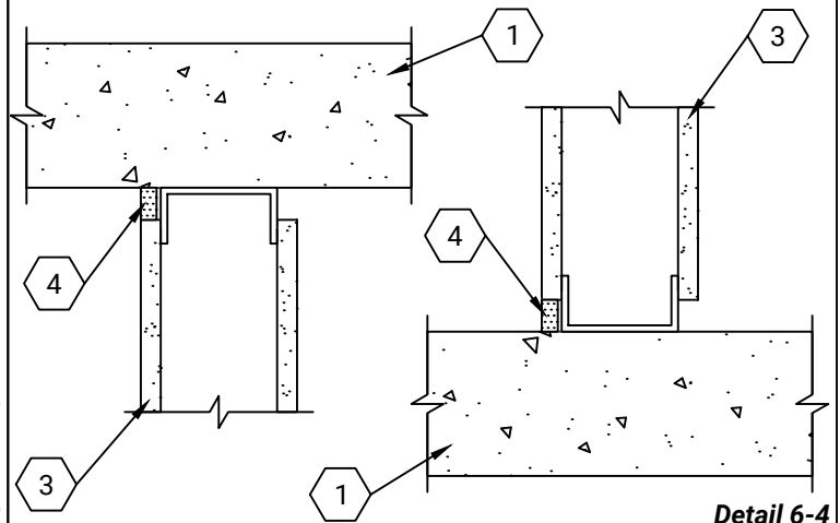
1/2" (12.7mm) Thickness - One Side of Wall
