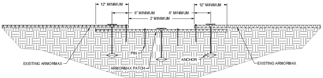
Figure 29: Armormax Patch Cross Section
