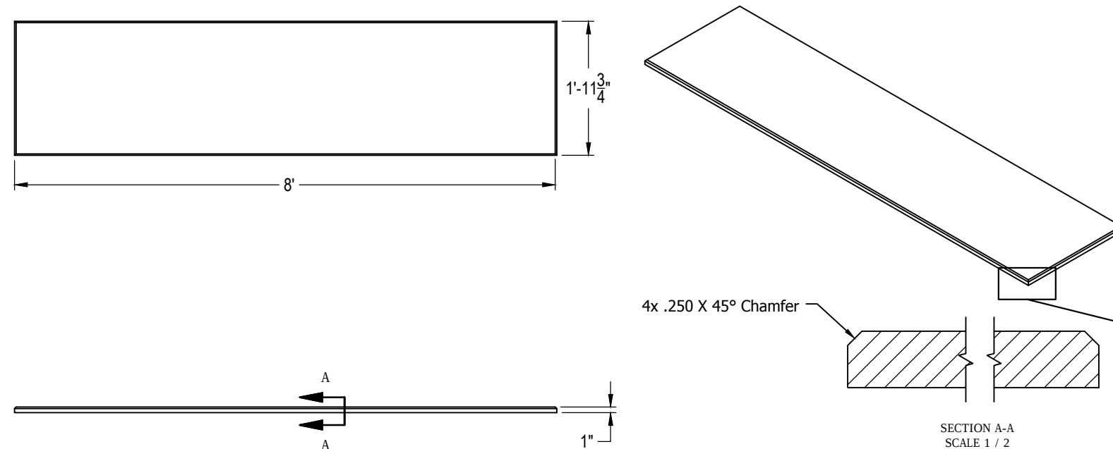
Tectum 1" Thick Direct Attach 24" x 96" Panel - BP8174T10
