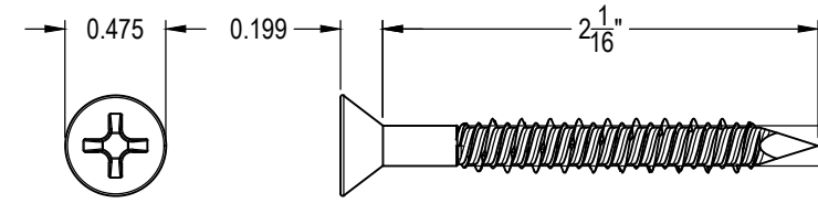
Tectum Direct Attach CMU Screw 1/4" Dia. x 2 1/4" - 8189L22
