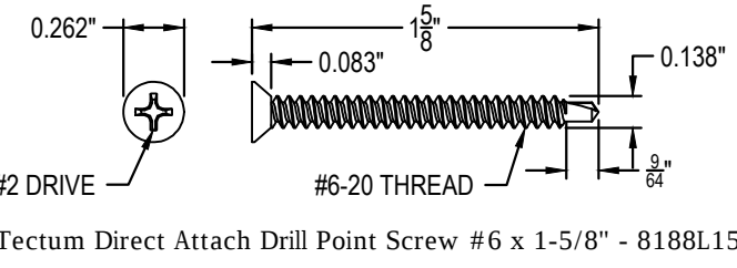
Tectum Direct Attach Drill Point Screw #6 x 1-5/8" - 8188L15
