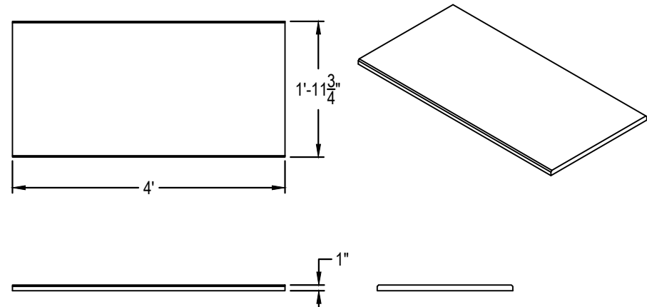
Tectum 1" Thick Direct Attach 24" x 48" Panel - BP8182T10
