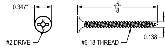
Tectum Direct Attach Sharp Point Screw #6 x 1-5/8" - 8187L15
