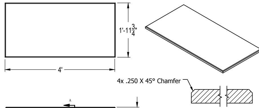
Tectum 1" Thick Direct Attach 24" x 48" Panel - BP8175T10
