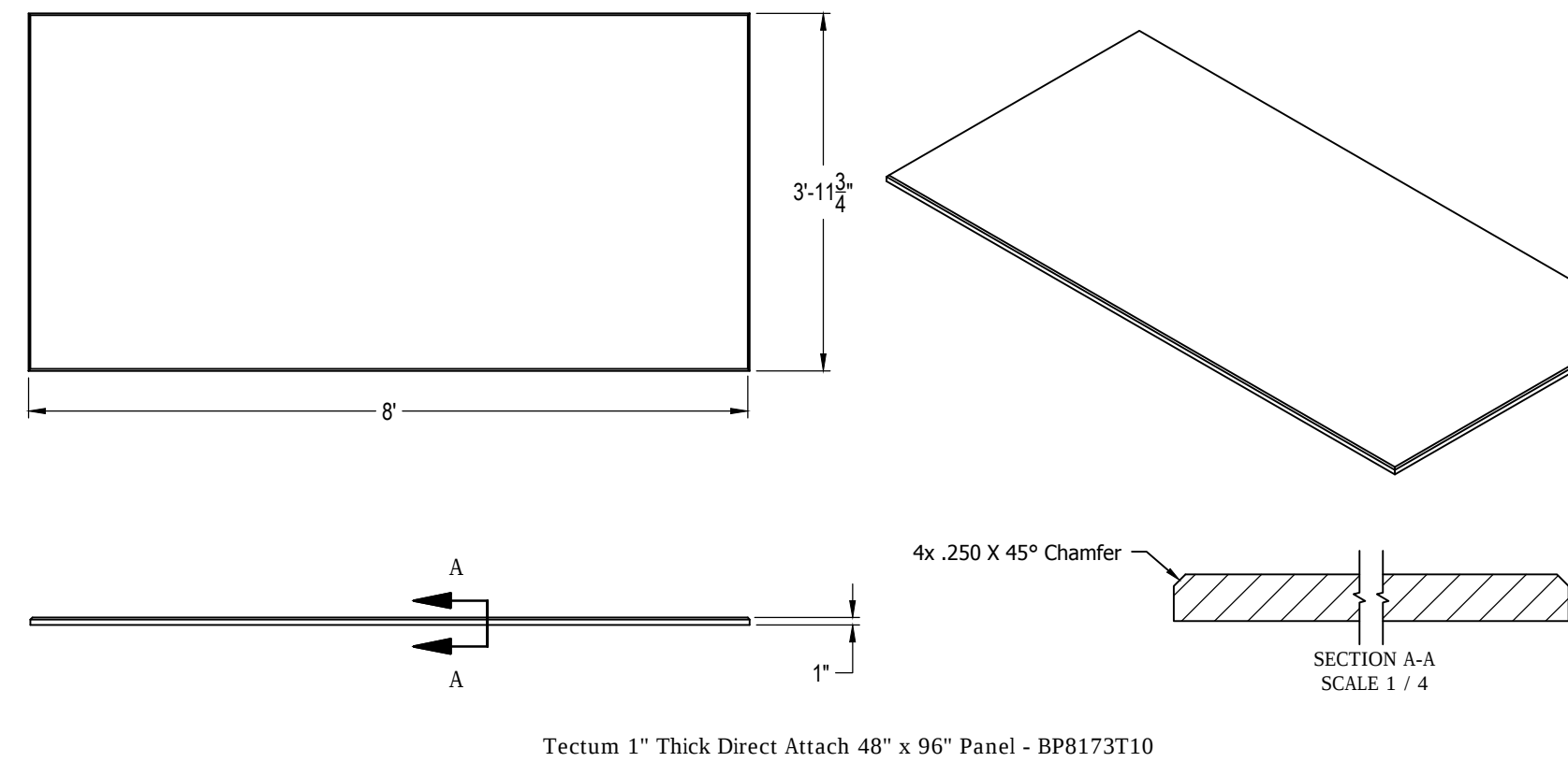
Tectum 1" Thick Direct Attach 48" x 96" Panel - BP8173T10
