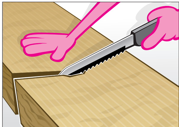
Cut Thermafiber® with long serrated knife
