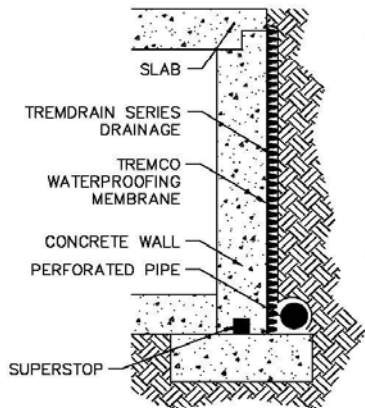
PIPE COLLECTION SYSTEM
