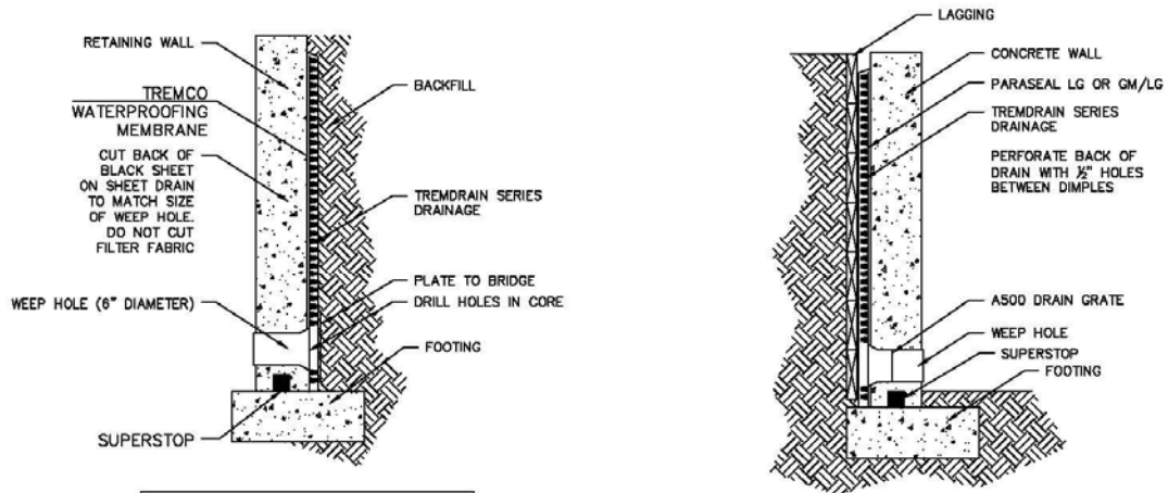
SHORING WALLS
