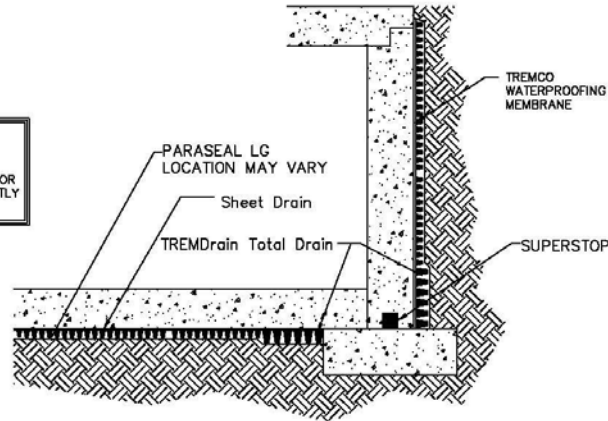
INSTALLATION UNDER SLABS
