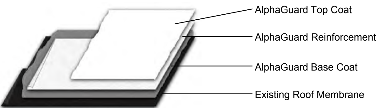
AlphaGuard Restoration System
