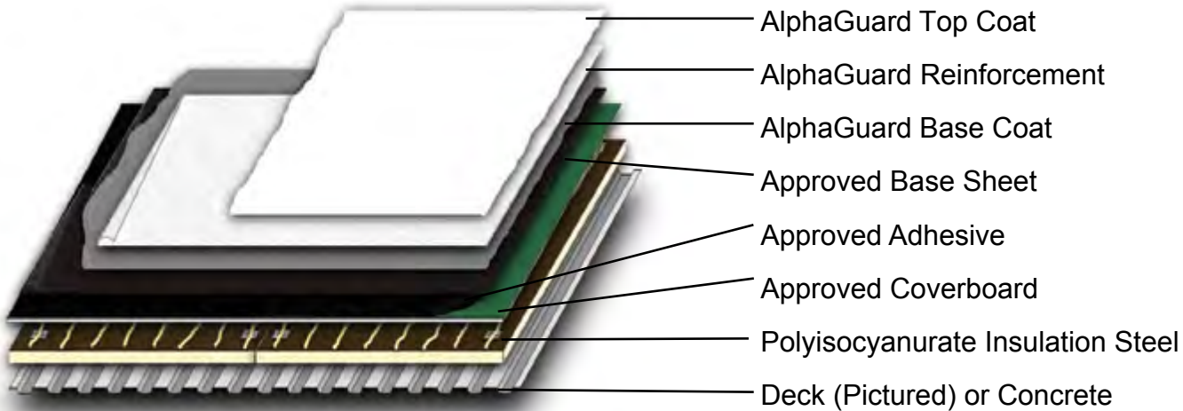
AlphaGuard Plus Roofing System
