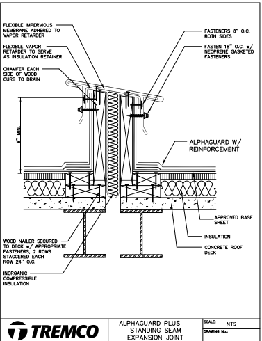
ALPHAGUARD PLUS STANDING SEAM EXPANSION JOINT
