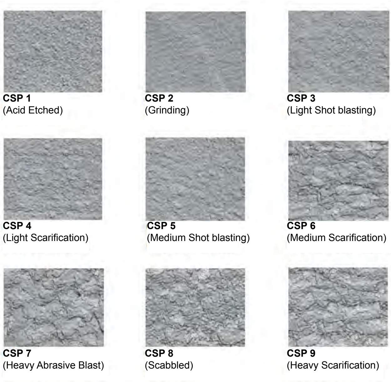
Surface profiles are provided by the International Concrete Repair Institute (ICRI). Molded replicas of these profiles can be purchased from ICRI at www.ICRI.org .
