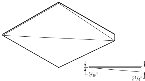
Geometrix® Outside Wedge Corner = GOC-2
