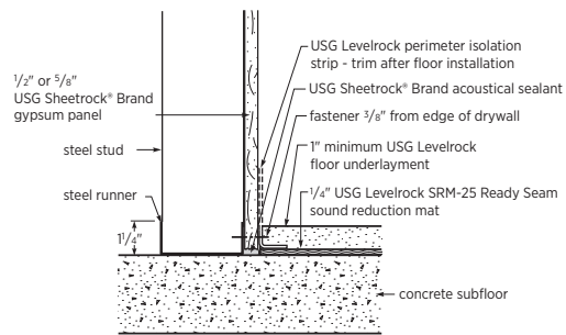
USG Levelrock SRM-25 Ready Seam Sound Reduction Mat Over Concrete USG Levelrock Poured After Drywall
