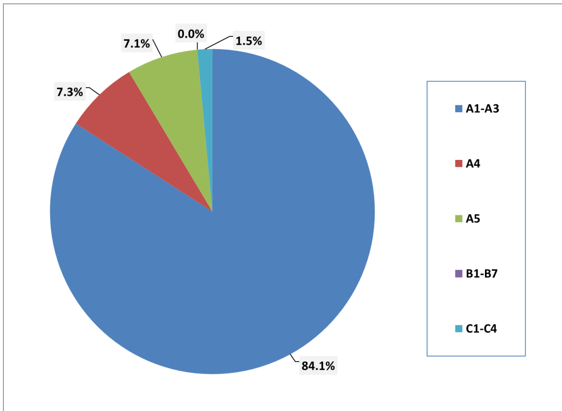
Figure 3: Process Dominance Analysis for GWP for the Production of 1 Square Foot of 3/4 in. Millennia™ Acoustical Ceiling Panels
