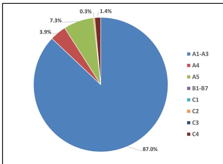
Figure 3: Process Dominance Analysis for GWP for the Production of 1 Square Foot of Radar™ High-NRC High-CAC SQ Acoustical Panels
