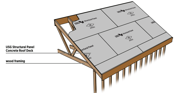
USG Structural Panel Concrete Roof Deck over Wood Truss.
