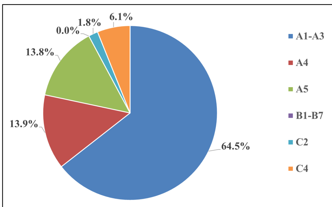
Figure 4: Process Dominance Analysis for the Production of 1 MSF of 5/8 in. (15.9 mm) Sheetrock® Brand EcoSmart Panels Firecode 30®
