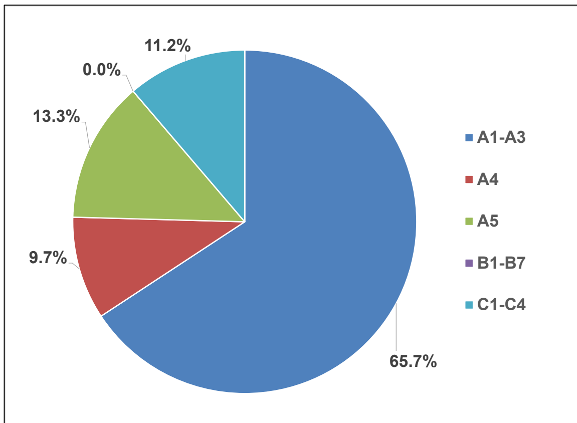
Figure 4: Process Dominance Analysis for the Production of 1 MSF of 5/8 in. (15.9 mm) Sheetrock® Brand EcoSmart Panels Mold Tough® Firecode® X
