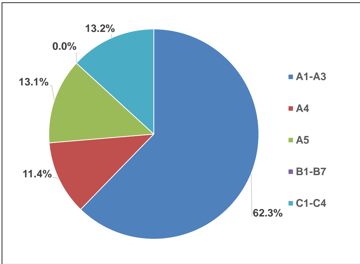
Figure 4: Process Dominance Analysis for the Production of 1 MSF of 5/8 in. (15.9 mm) Sheetrock® Brand Firecode® X Panels
