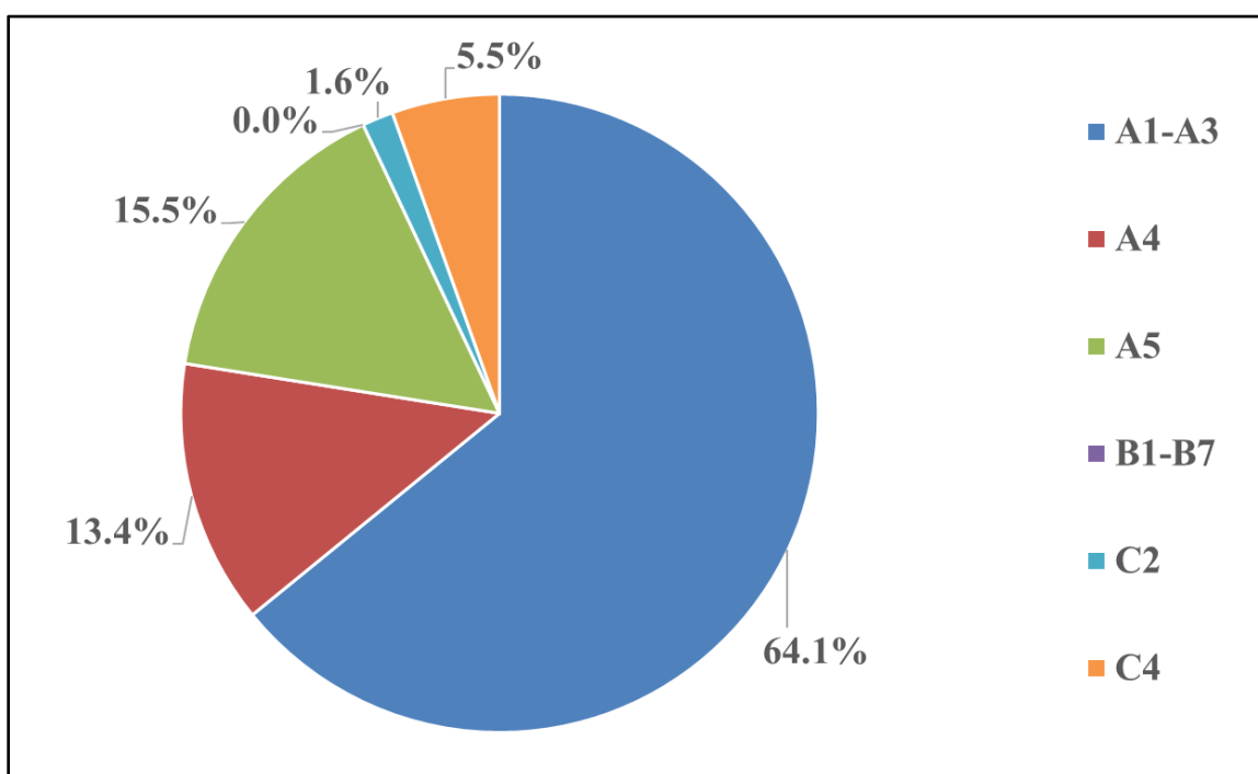
Figure 4: Process Dominance Analysis for the Production of 1 MSF of 1/4 in. (6.4 mm) Sheetrock® Brand Gypsum Panels
