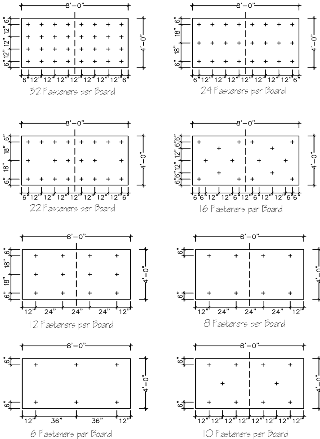
Figure 1 - Fastener layout
