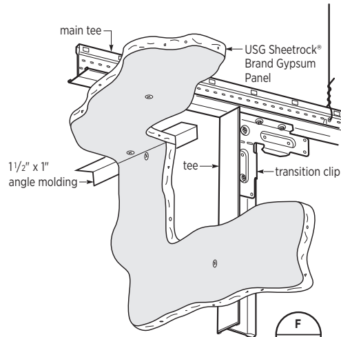
90° inside corner
