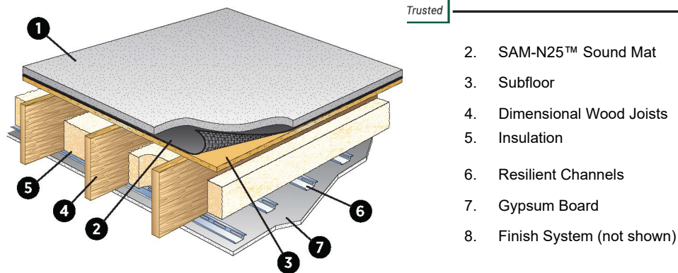
FIGURE 7—SOUND TRANSMISSION RATED FLOOR/CEILING ASSEMBLY—SEE TABLE 4 FOR ASSEMBLIES 4—6
