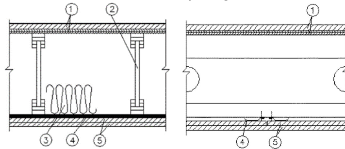
Fire Resistance Ratings - ANSI/UL 263 Unrestrained Assembly Rating — 1 Hour
