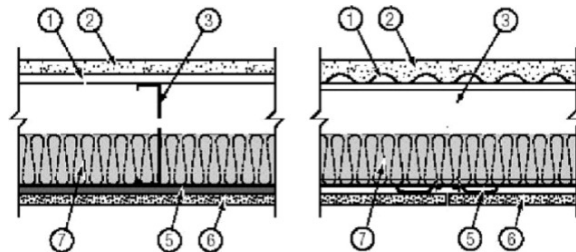
Fire Resistance Ratings - ANSI/UL 263 Unrestrained Assembly Rating — 1 Hour or 2 Hour
