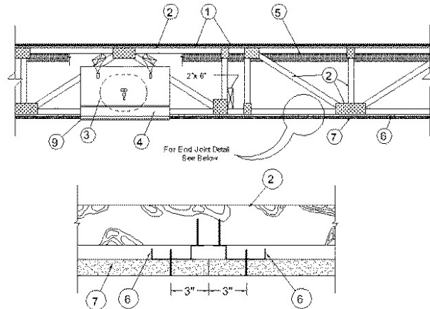
FIGURE 3—1-HOUR FLOOR/CEILING ASSEMBLY CONSTRUCTED WITH OPEN WEB WOOD TRUSSES
