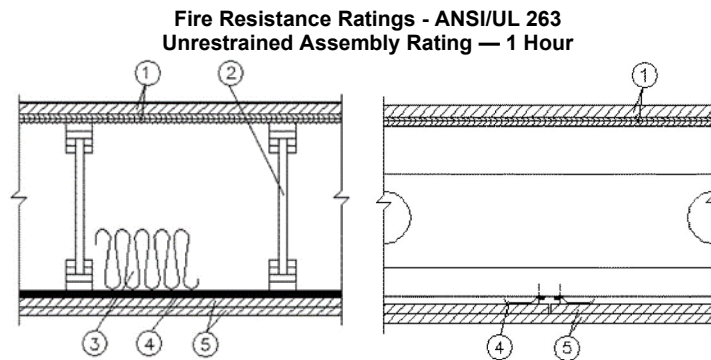
FIGURE 1—1-HOUR FLOOR/CEILING ASSEMBLY CONSTRUCTED WITH WOOD I-JOISTS
