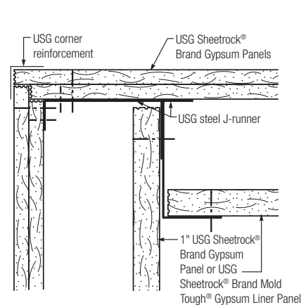
Outside Corner
