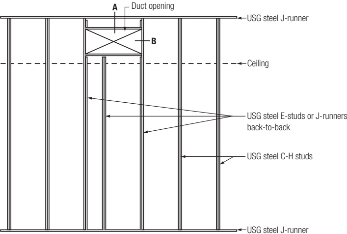
Typical Duct Opening Penetration (See Damper and Duct Manufacturer Installation Instructions for Further Details)
