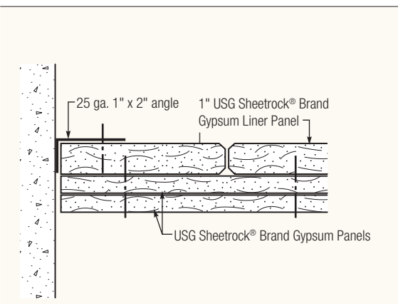
Wall Intersection
