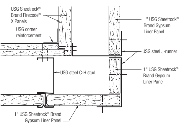
Inside Corner
