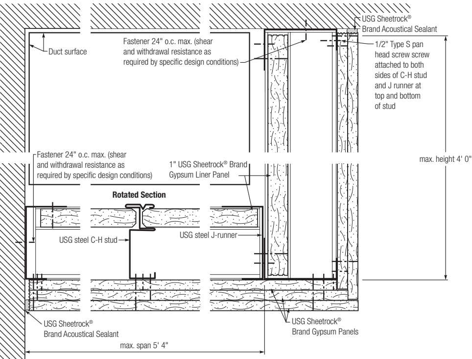
Two-Hour Rated Assembly – Horizontal Membrane or Metal Duct Enclosure
