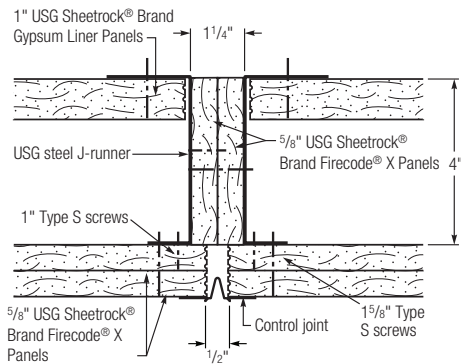
Control Joint in Two-Hour Shaft Walls
