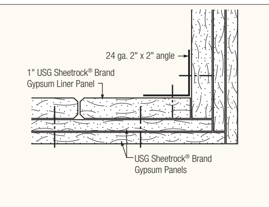
Corner
