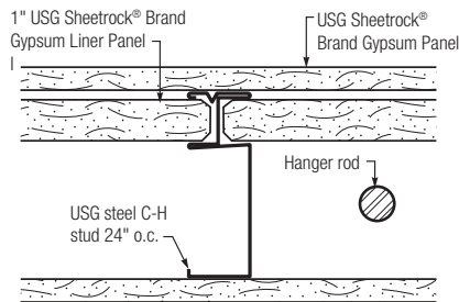
Cross-Section at Stair Hanger
