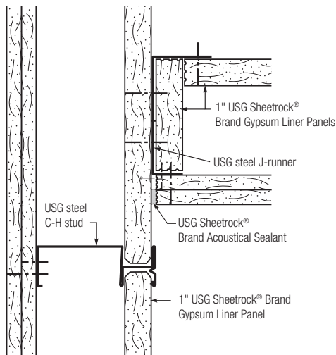
Wall Junction
