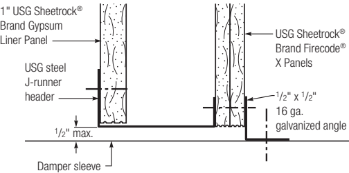
Section A: Fire Damper Installation (See Damper and Duct Manufacturer Installation Instructions for Further Details)
