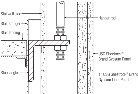
Stair Hanger and Rod Application
