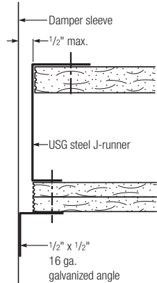
Section B: Fire Damper Installation (See Damper and Duct Manufacturer Installation Instructions for Further Details)
