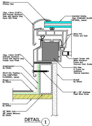
HORIZONTAL CROSS SECTION
