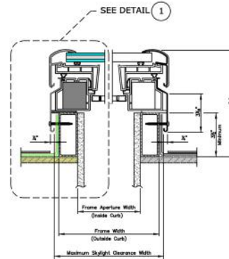
HORIZONTAL CROSS SECTION
