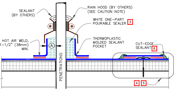
TPC-16.1 Molded Sealant Pocket
