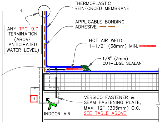
TPC-12.1 Parapet Flashing
