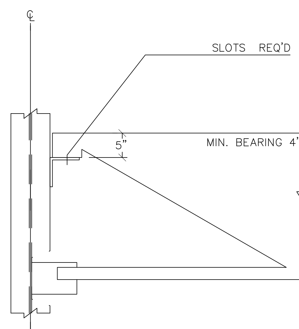
J49 ON SIDE OF W - FLANGE COLUMN
