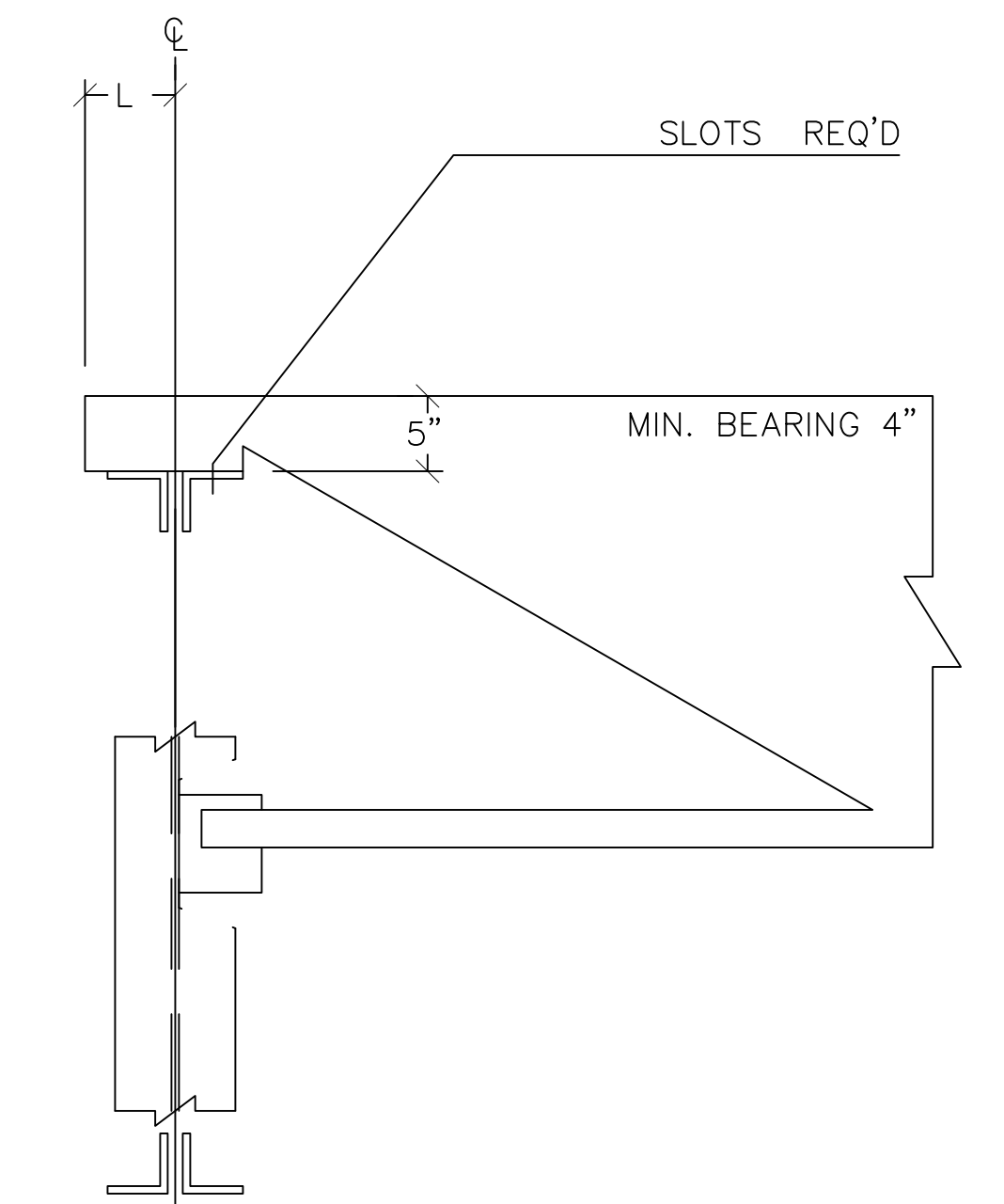
J41 ON GIRDER AT W-FLANGE COLUMN W/ TCX
