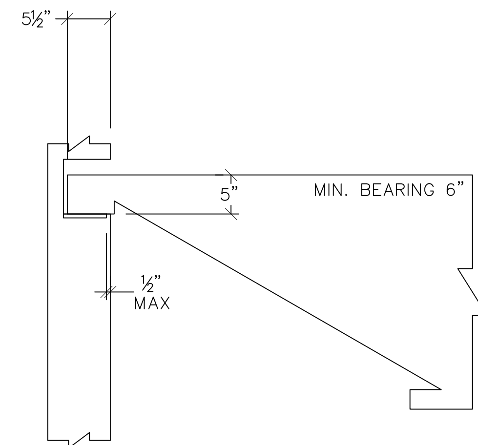
J44 IN WALL POCKET
