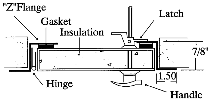
SECTION DETAIL
