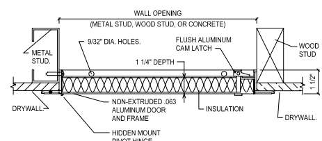
SECTION DETAIL:
