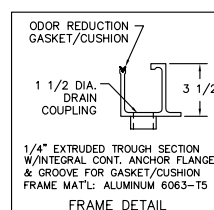
SECTION DETAIL:
