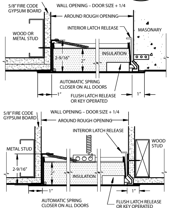
Ultra Lock w/2 keys
