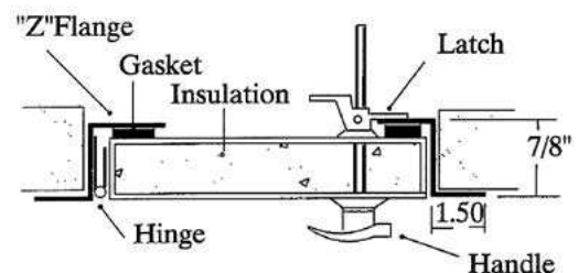
SECTION DETAIL:
