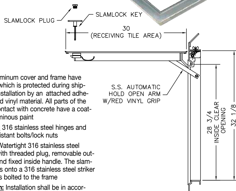
SECTION DETAIL:
