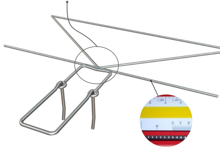
ASTM A 951 Deformations 8 sets/inch
