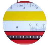
ASTM A 951 Deformations 8 sets/inch
