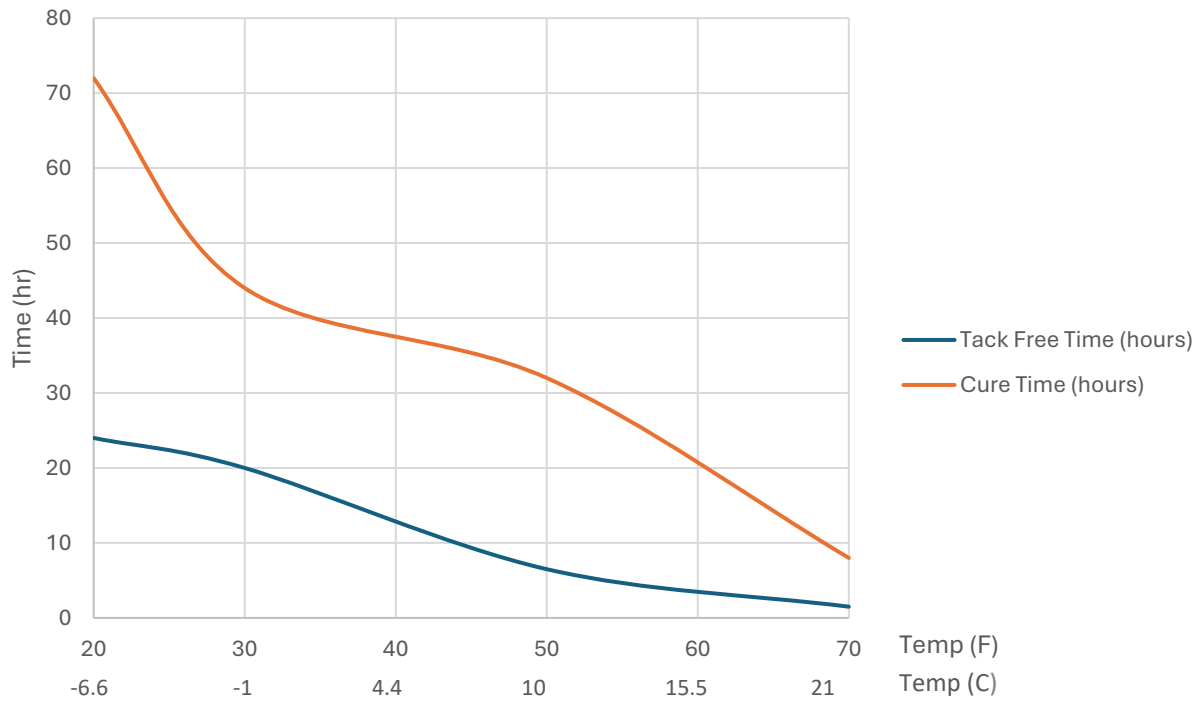
POINTING MASTIC Tack-Free and Cure Times
