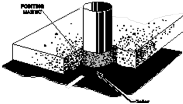
PROFILION DETAIL
